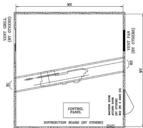
PLAN OF HOISTWAY & MACHINE ROOM
